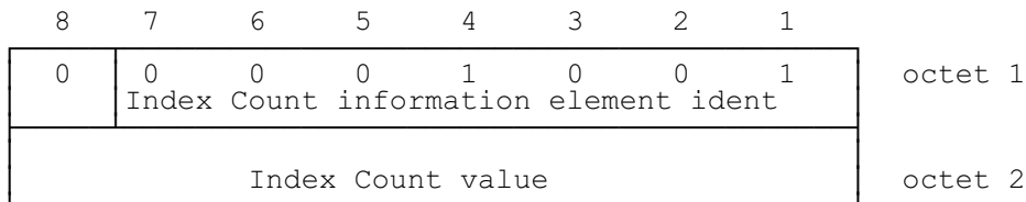
Figure 2.5.11/GSM 07.05: Index Count information element
