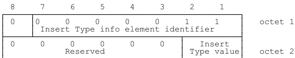
Figure 2.5.5/GSM 07.05: Insert Type information element
