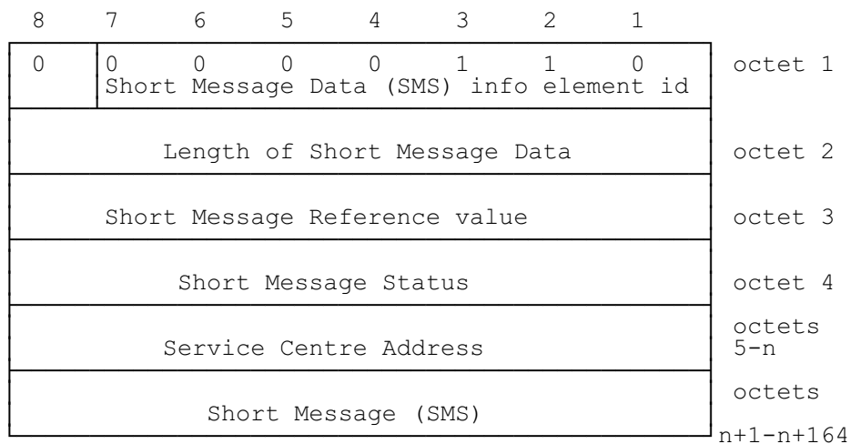
Figure 2.5.8/GSM 07.05: Short Message Data (SMS) information element
