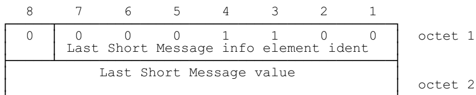
Figure 2.5.14/GSM 07.05: Last Short Message information element
