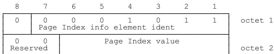
Figure 2.5.13/GSM 07.05: Page Index information element
